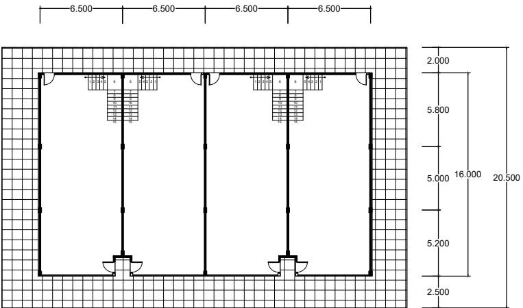
Lantai 1
