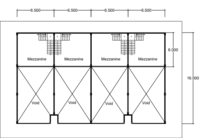
Lantai Mezzanine
